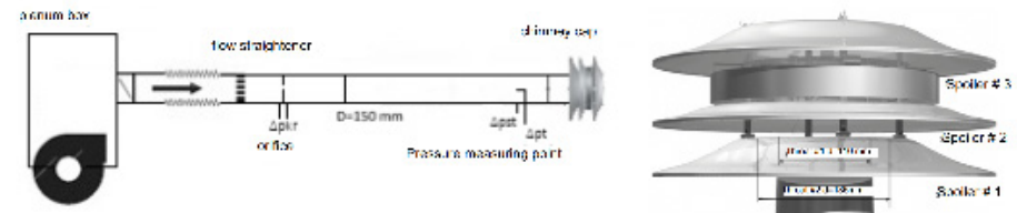
Figure 1 Test stand layout and chimney cap
